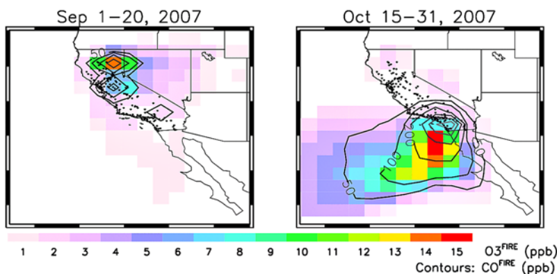
Figure 1. Mean modeled surface mixing ratios (ppb) for \text{O}_3^{\text{FIRE}} (filled contours) and \text{CO}^{\text{FIRE}} (contour lines) for (left) September 1–20 and (right) October 15–31. Dots indicate the locations of EPA monitoring sites.
